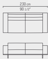
3 Seater 230 cm PBC 06.105.01.--
